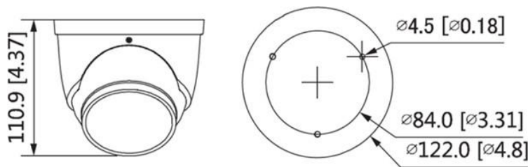
Figure 3-1. Dimensions (unité : mm [pouces])
