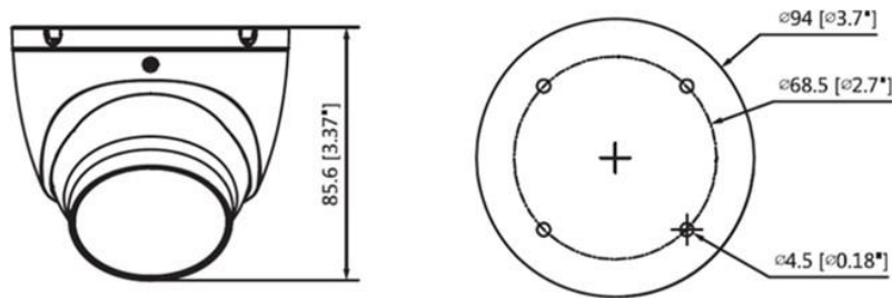
Figure 3-1. Dimensions (unité : mm [pouces])
